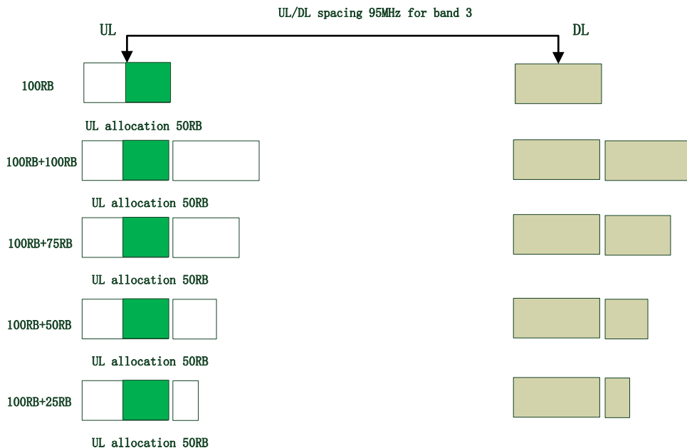
Figure 6.2.2 UL allocation for CA band 3 in TS 36.101 when testing REFSENS
